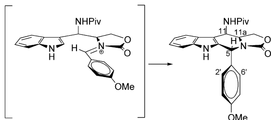
Figure 4. Stereoselectivity model for the Pictet–Spengler reaction.
