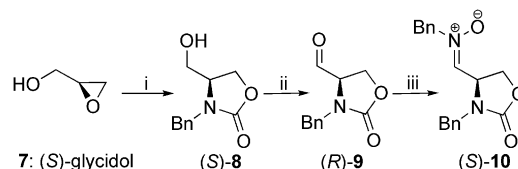
Scheme 1. Enantioselective synthesis of the nitrone ( S )- 10 . Reagents and conditions: (i) \text{BnNCO} (1 equiv.), \text{Et}_3\text{N} (1.8 equiv.), \text{CH}_2\text{Cl}_2 , 40 °C, 18 h (74%); (ii) DMP (2 equiv.), \text{CH}_2\text{Cl}_2 , room temp., 1.5 h (60%), or IBX (3 equiv.), \text{EtOAc} , 80 °C, 3 h (quant.); (iii) \text{BnNHOOH} (1.7 equiv.), \text{MgSO}_4 (excess), \text{CH}_2\text{Cl}_2 , room temp., 3 h (98%).
