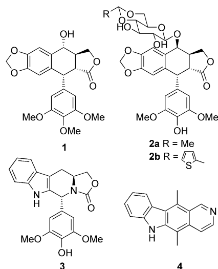
Figure 1. Structures of bioactive lignans and ellipticine: podophyllotoxin ( 1 ), etoposide ( 2a ), teniposide ( 2b ), azaelliptitoxin ( 3 ), ellipticine ( 4 ).
