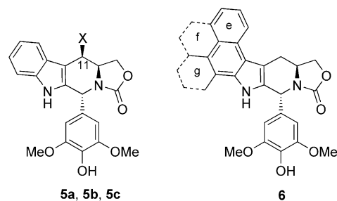
Figure 2. Structures of some azaelliptitoxin derivatives: 5a (X = OR), 5b (X = NHR 1 ), 6 (benz[e, f] and glazaelliptitoxins).
